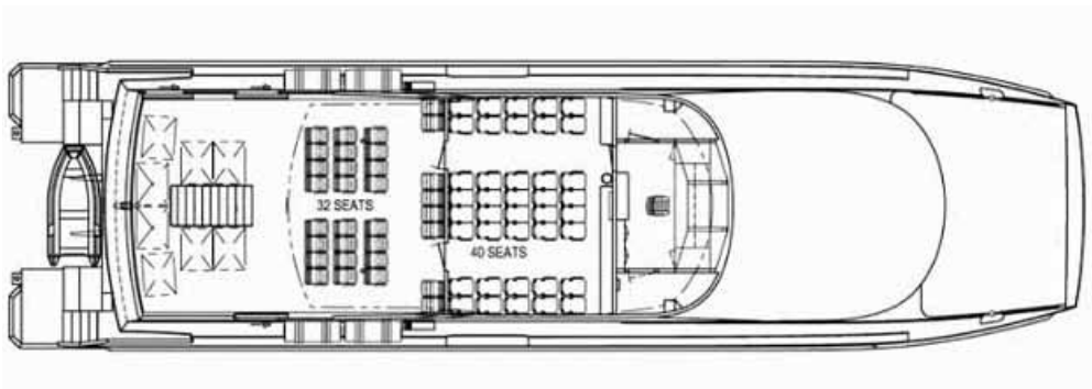
UPPER DECK
